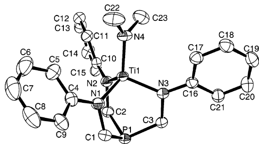
Figure 3. Solid-state molecular structure of 2b as determined by X-ray crystallography. Hydrogen atoms are omitted for clarity. Selected distances (Å): Ti(1)···P(1), 2.9895(4); Ti(1)–N(1), 1.9239(11); Ti(1)–N(2), 1.9327(11); Ti(1)–N(3), 1.9424(11); Ti(1)–N(4), 1.8643(12). Selected bond angles: C(1)–P(1)–C(2), 105.85(6); C(1)–P(1)–C(3), 102.64(6); C(2)–P(1)–C(3), 102.89(6); Ti(1)–N(4)–C(22), 130.95(11); Ti(1)–N(4)–C(23), 115.22(10); Ti(1)–N(1)–C(1), 109.48(8); Ti(1)–N(1)–C(4), 132.54(9); Ti(1)–N(2)–C(2), 108.78(8); Ti(1)–N(2)–C(10), 133.75(9); Ti(1)–N(3)–C(3), 109.80(8); Ti(1)–N(3)–C(16), 134.33(9); P(1)–C(1)–N(1), 116.64(9); P(1)–C(2)–N(2), 118.59(9); P(1)–C(3)–N(3), 117.06(9); C(1)–N(1)–C(4), 117.13(11); C(2)–N(2)–C(10), 117.47(11); C(3)–N(3)–C(16), 115.74(10).
