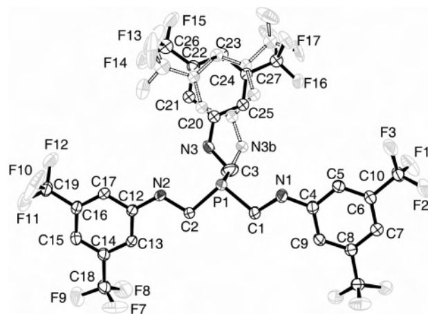
Figure 2. ORTEP depiction of the solid-state structure of 1a as determined by X-ray crystallography. Selected bond angles: C(1)–P(1)–C(2), 99.48(11)^\circ ; C(1)–P(1)–C(3), 99.38(15)^\circ ; C(2)–P(1)–C(3), 100.59(16)^\circ ; P(1)–C(1)–N(1), 107.99(18)^\circ ; P(1)–C(2)–N(2), 107.79(16)^\circ ; C(1)–N(1)–C(4), 123.7(2)^\circ ; C(2)–N(2)–C(12), 120.95(19)^\circ .
