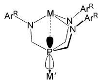
Figure 1. Potential binding mode of the of P(\text{CH}_2\text{NAr}^R)_3 ligands to an early transition metal fragment (shown as M) and a second metal complex (shown as M') along with an illustration of the major and minor lobes of the lone pair orbital on phosphorus.
